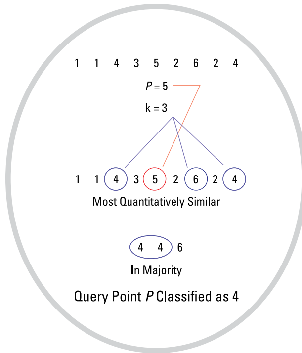
FIGURE 5-10: How kNN works.
