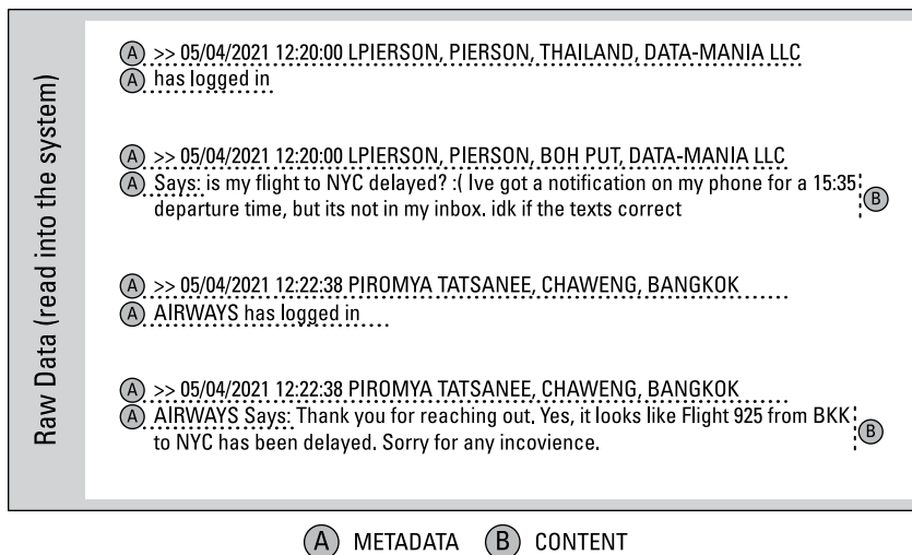
FIGURE 13-3: An example of raw data ingested into an NLP system.
