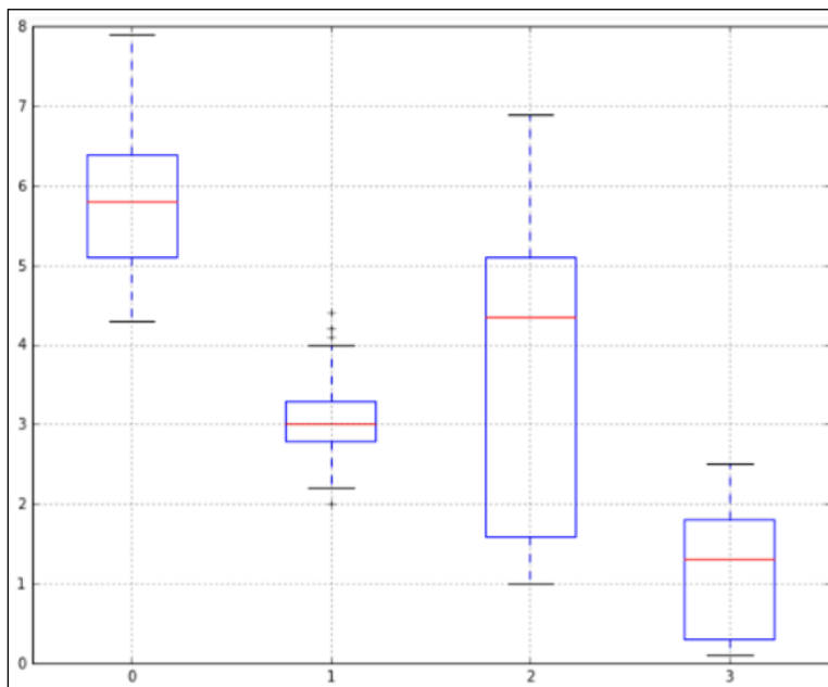
FIGURE 4-7: Spotting outliers with a Tukey boxplot.
