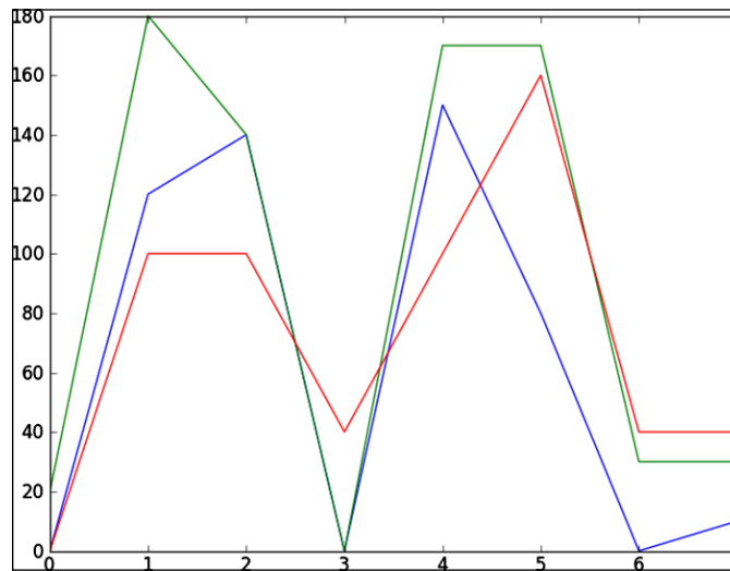
FIGURE 6-2: Time-series plot of monthly snow depth data.
