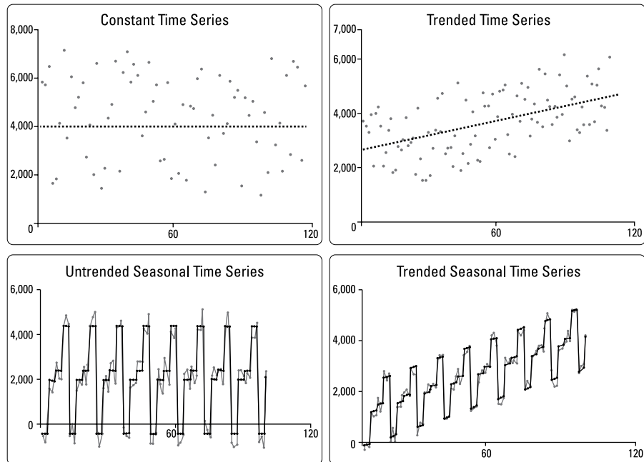
FIGURE 4-9: A comparison of patterns exhibited by time series.
