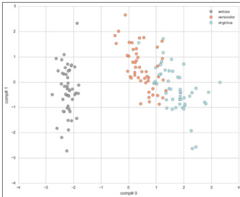
FIGURE 8-16: A scatterplot.
