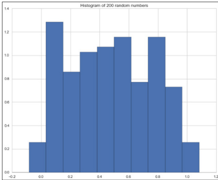
FIGURE 8-15: A histogram.
