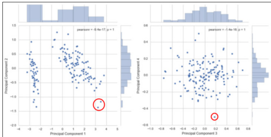
FIGURE 4-8: Using PCA to spot outliers.
