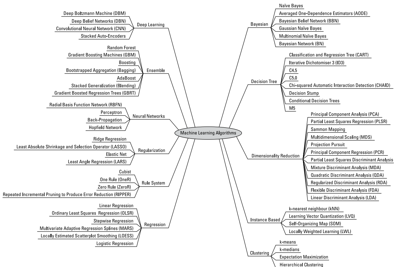
FIGURE 3-3: Machine learning algorithms can be broken down by function.
