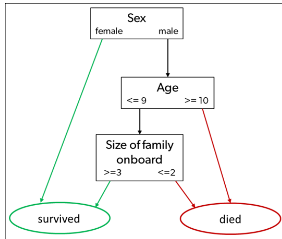
FIGURE 5-6: A decision tree model predicts survival rates from the Titanic catastrophe.
